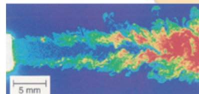
Tomographic Image of a Jet
