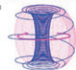
Magnetic field line is closed by the plasma current and confines the plasma.
