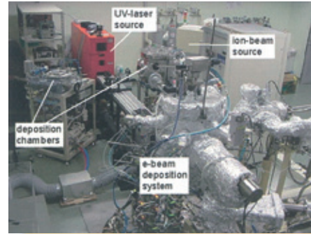
Electron-beam deposition and pulsed-laser deposition systems for fabrication of high-quality thin films
