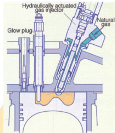
Direct Injection Gas Engine
